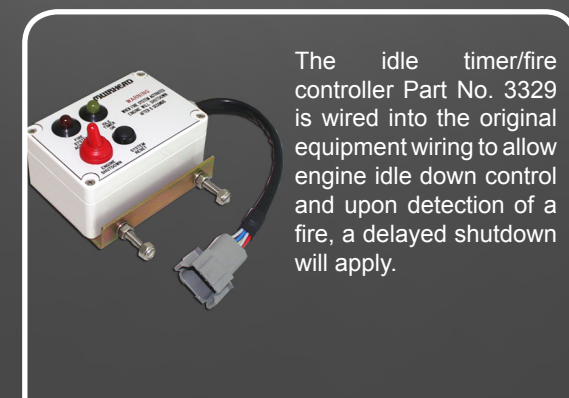
Part No. 3329 Idle timer/fire controller 24V
